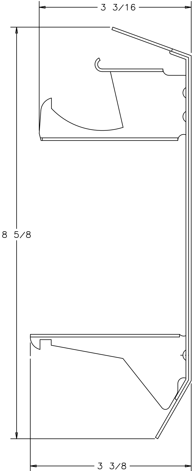
80 Bracket
